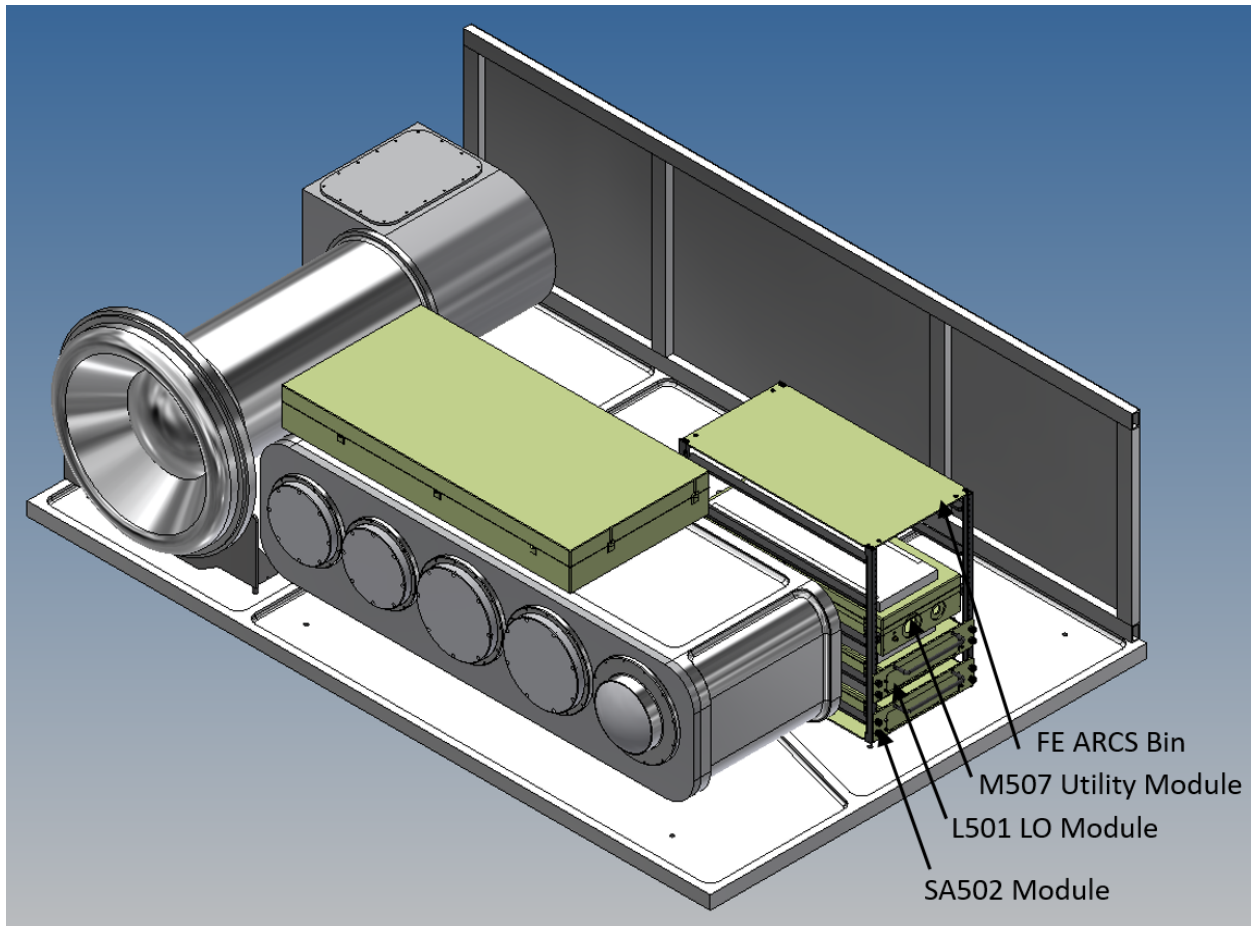
Figure 12. Populated FE Enclosure Overview, Bin and Modules Detail
