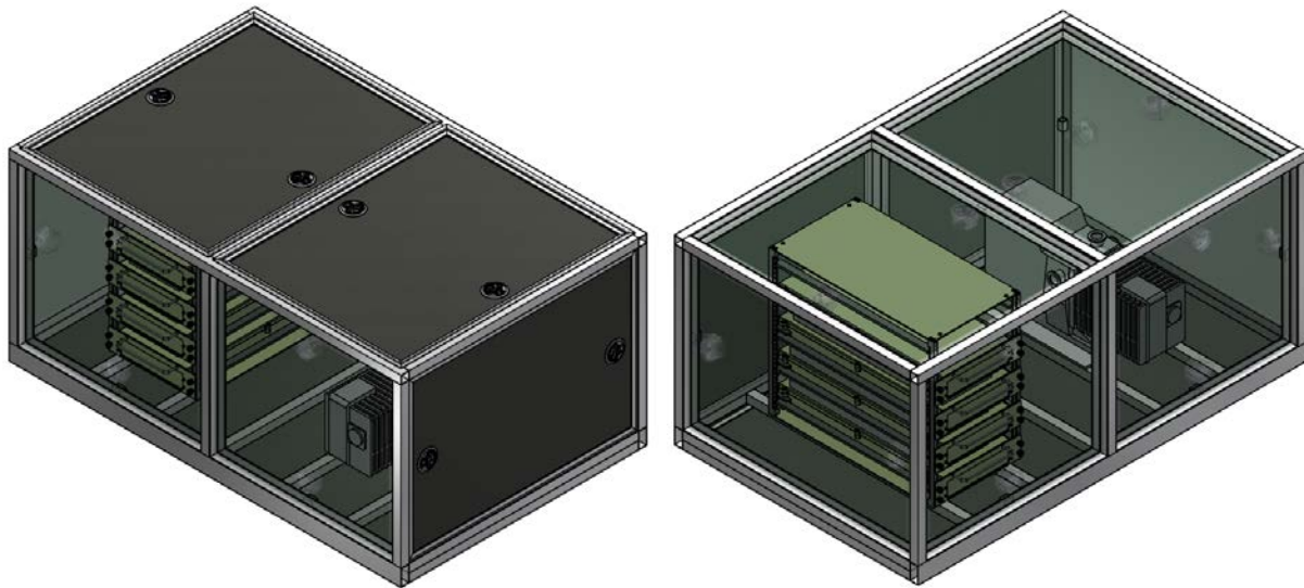
Figure 13. Auxiliary Enclosure Overview
