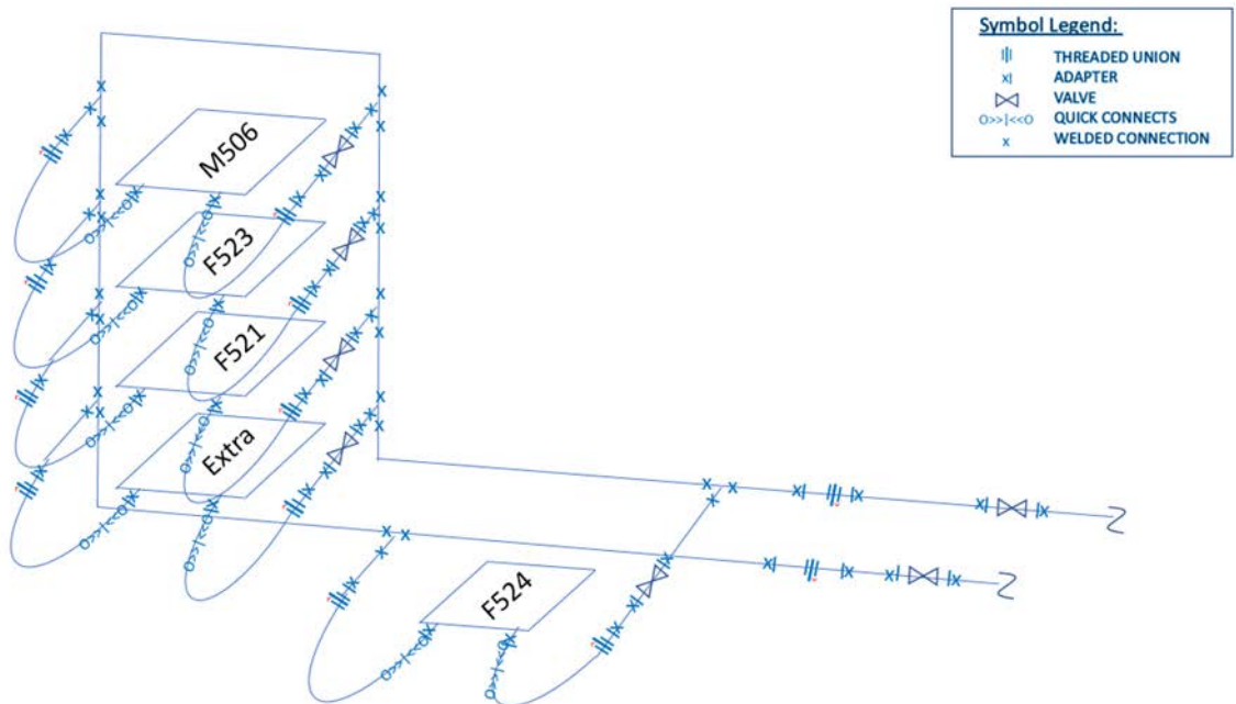
Figure 19. Auxiliary Enclosure Piping Diagram
