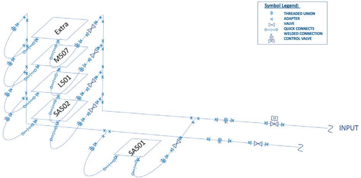
Figure 18. Front End Enclosure Piping Diagram
