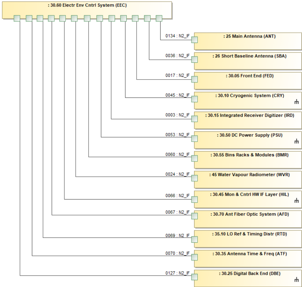
Figure 4. EEC External Interfaces
