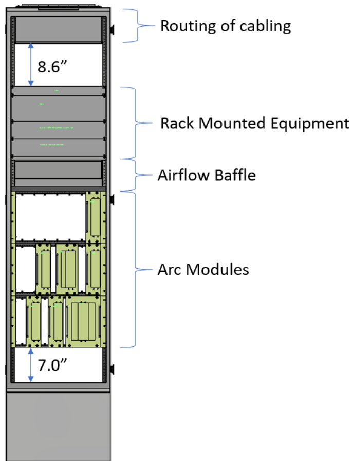
Figure 16. Electronics Rack Layout, front view
