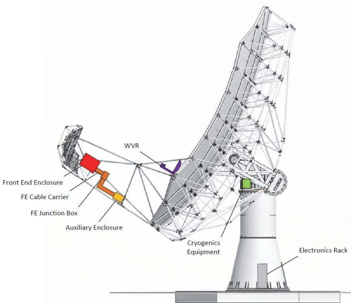
Figure 1. Antenna Electronics Primary Locations
