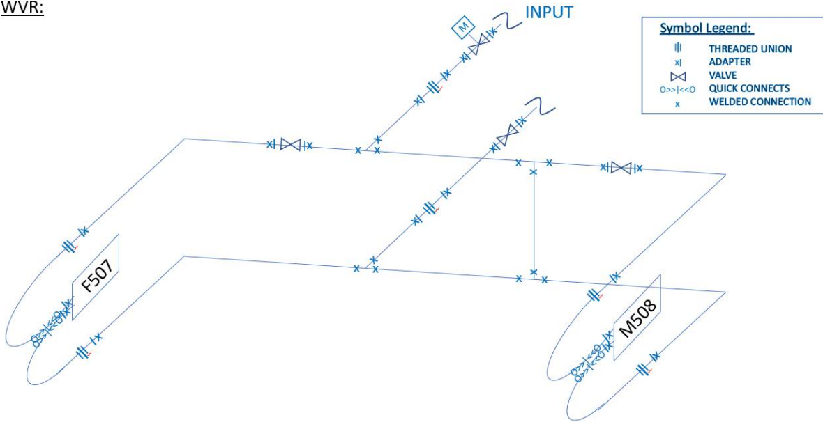
Figure 20. WVR Piping Diagram
