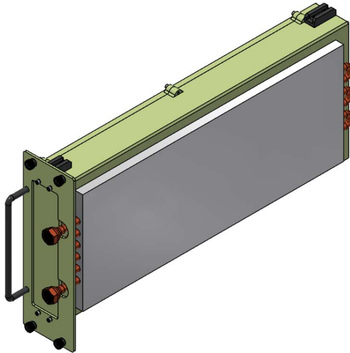
Figure 8. ARCS Module with cold plate, disconnected from the glycol system
