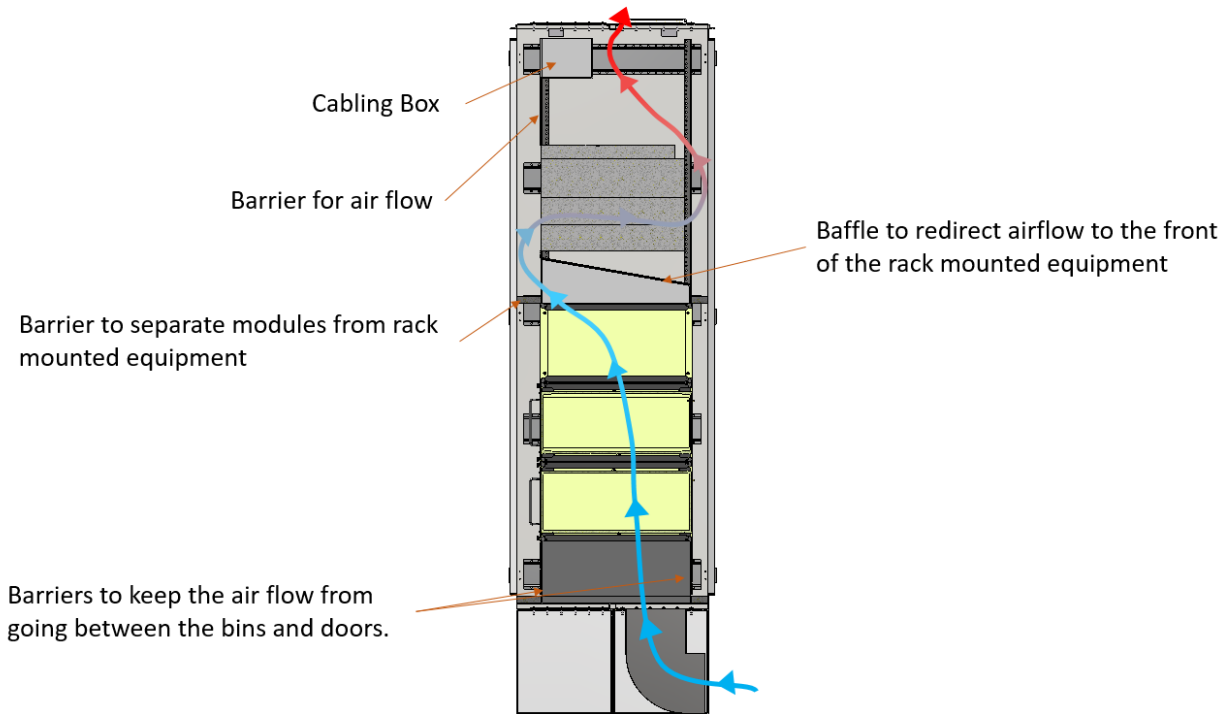
Figure 17. Electronics Rack Air Flow, side section view
