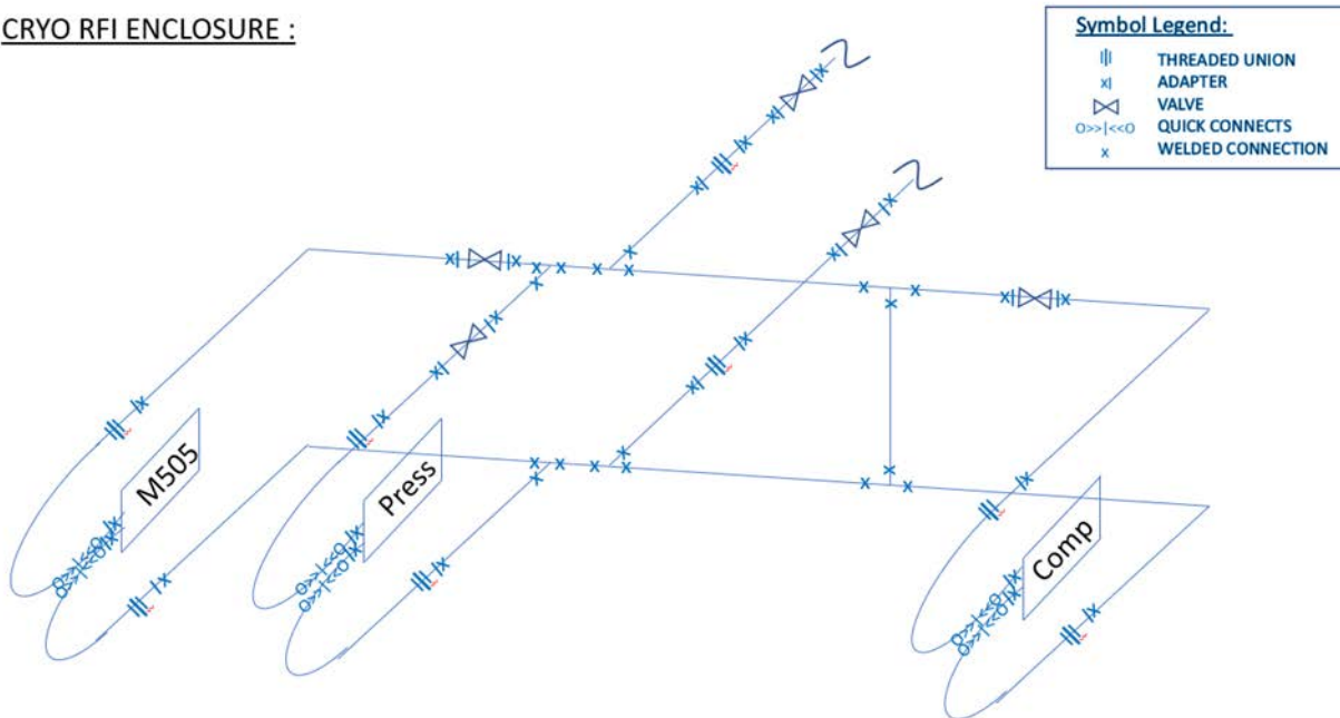
Figure 21. Cryogenics RFI Enclosure Piping Diagram
