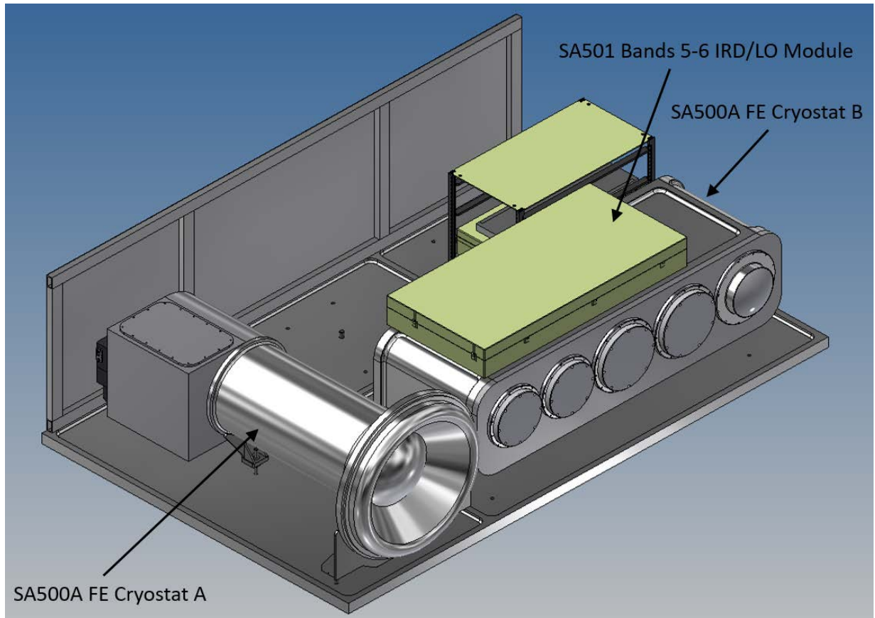
Figure 11. Populated FE Enclosure Overview, Cryostats and IRD/LO Enclosure
