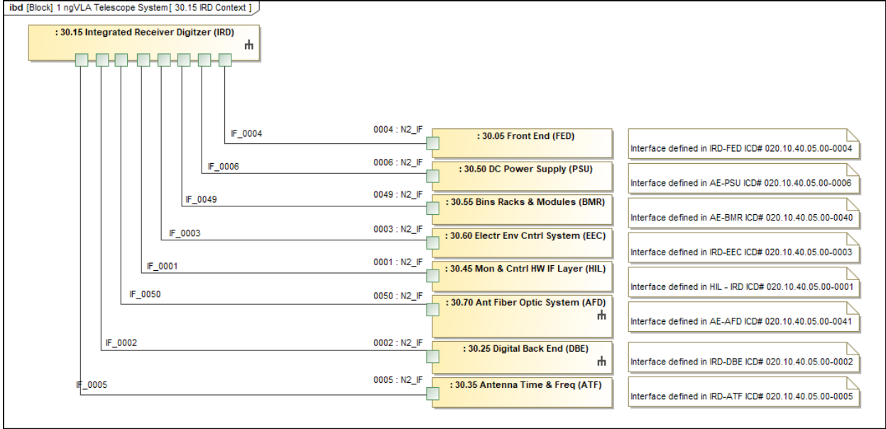
Figure 1: SysML Representation of the IRD subsystem.
