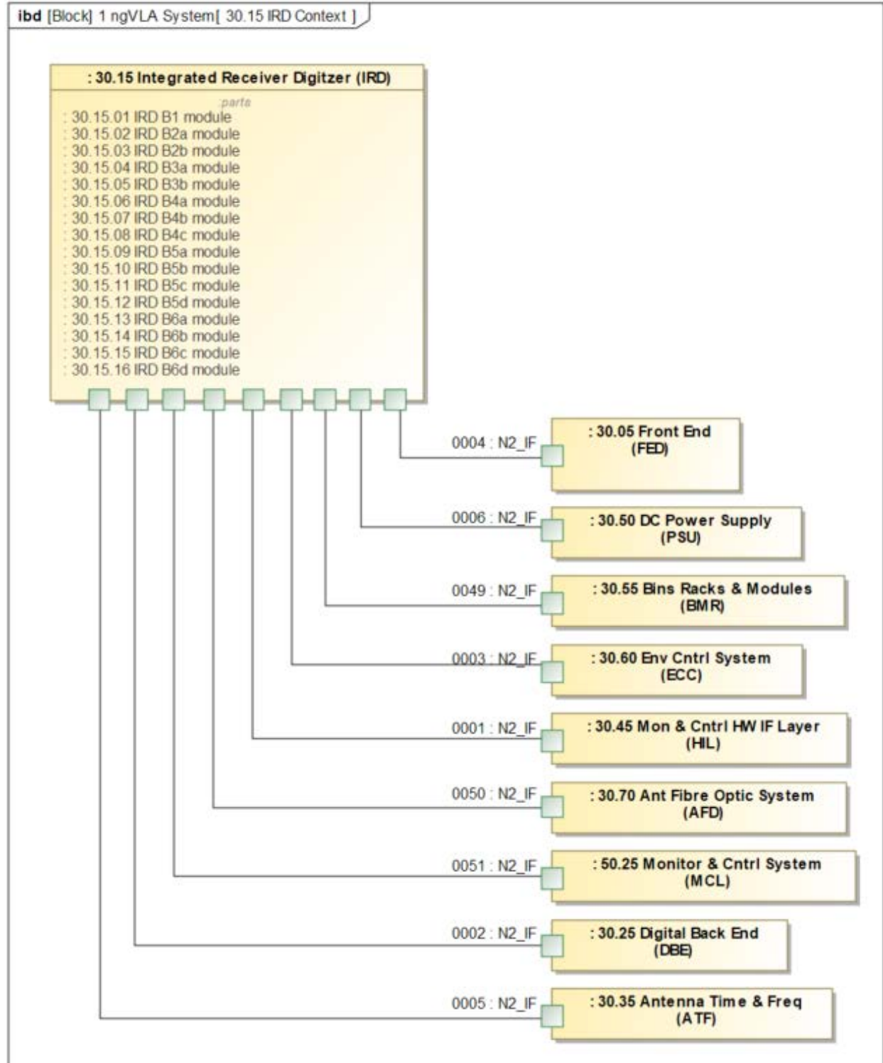
Figure I: SysML Representation of the IRD subsystem.
