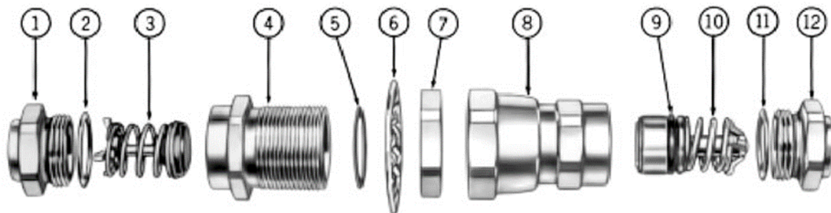
Typical Male Coupling Half (S2)
