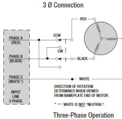
Figure 36: Sumitomo CH-204SFF 3-phase AC synchronous motor, 72 rpm at 60 Hz, 208VAC 3-phase.
