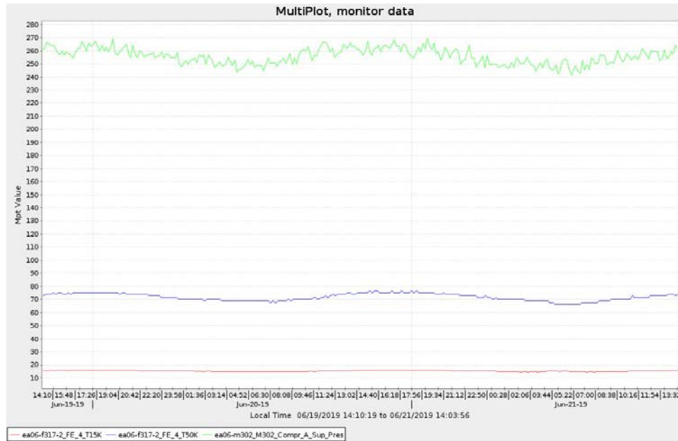
Figure 13: Example of diurnal pressure variation on Antenna 6 Q-band (VLA June 2019).
