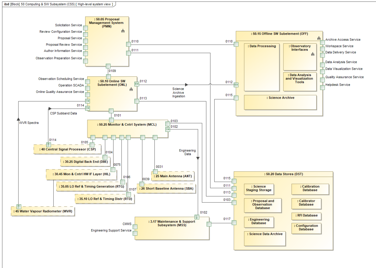
Figure 37 - Internal block diagram of the Computing & Software System.
