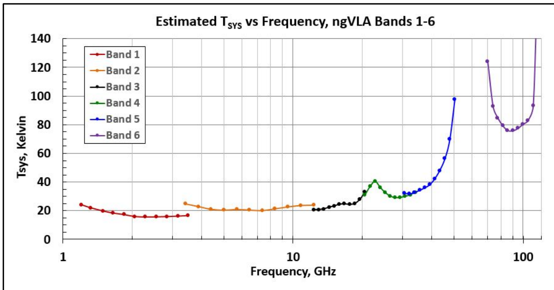
Figure 18 - System temperature for the ngVLA 6-band receiver configuration.
