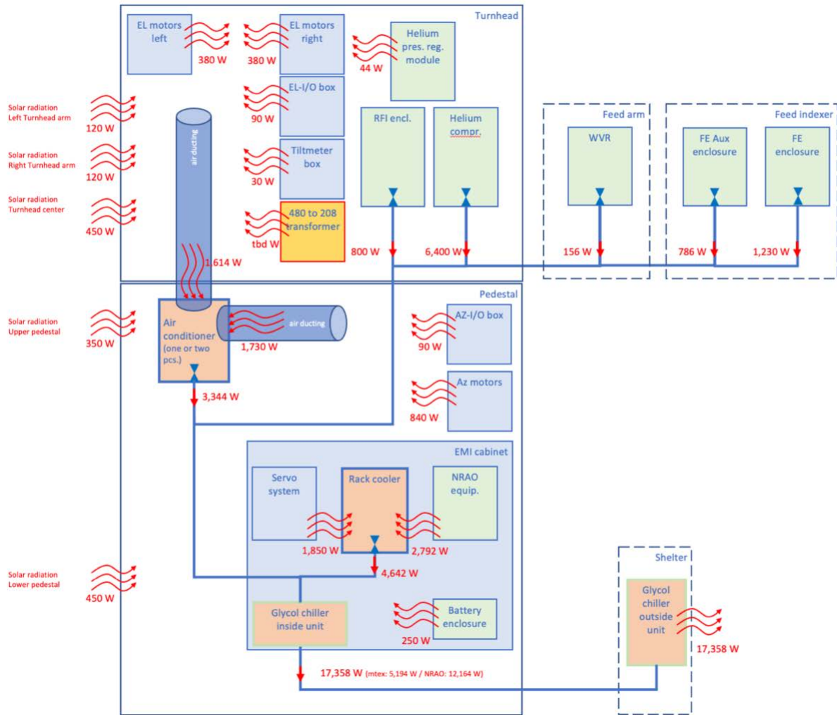
Figure 29 - Overview of the antenna environmental control system and associated heat loads.
