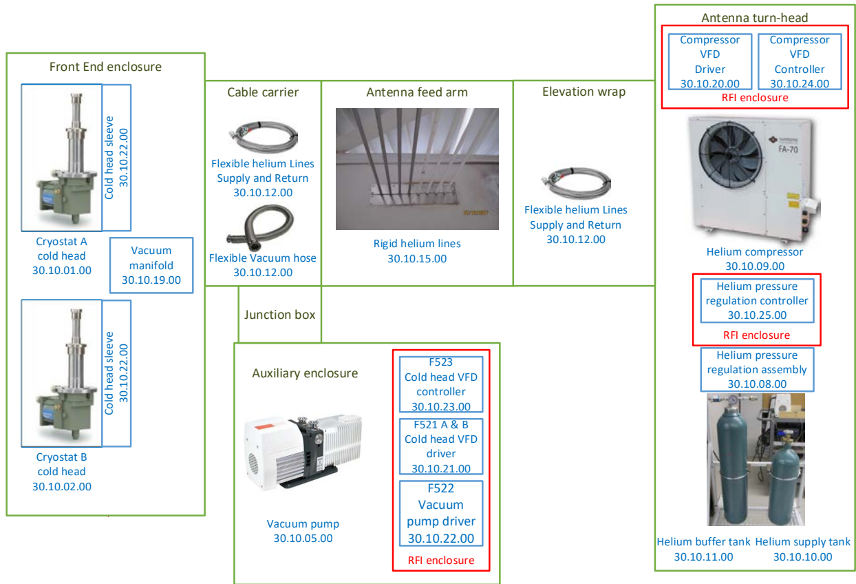
Figure 20 - Cryogenic system block diagram. Part numbers within the product breakdown structure are also given [AD25].
