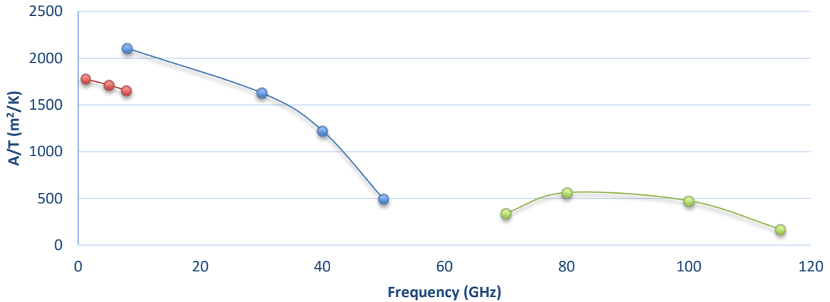
Figure 2 - System A/T specification in m 2 /K. (SYS1001)
