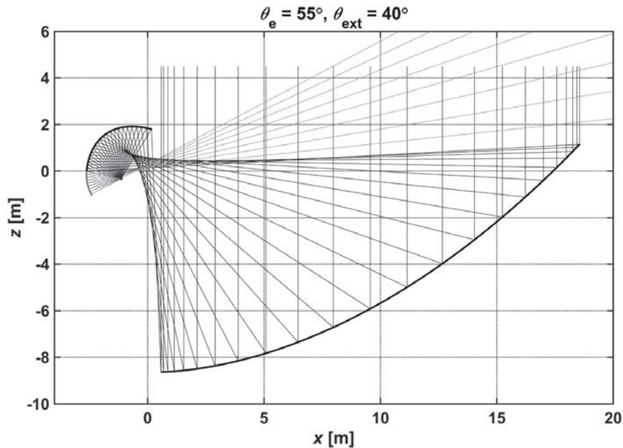
Figure 15 - Optical baseline design that will be used for the antenna preliminary design and prototype.
