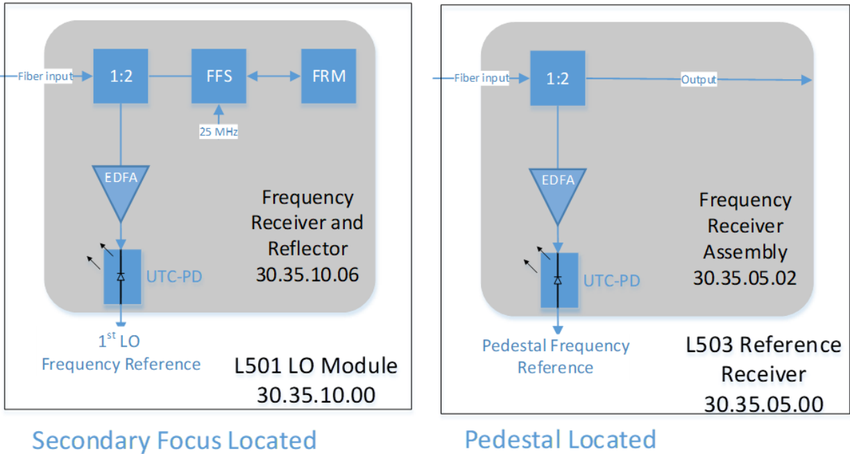
Figure 32 – Left: Frequency Transfer Link LO Reference Receiver and Reflector. Right: LO reference for pedestal-based electronics. FFS = fiber frequency shifter, FRM = Faraday rotator mirror, EDFA = erbium-doped fiber amplifier, UTC-PD = uni-traveling carrier photodiode.
