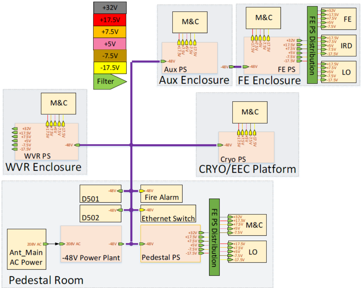
Figure 25 - Block diagram of the DC power supply system.
