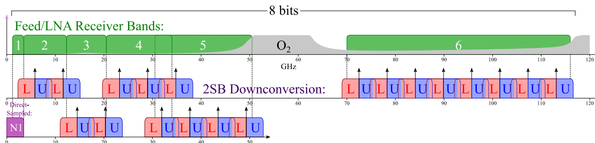
Figure 22 – downconverter-digitizer concept employing integrated receiver technology for both direct and dual sideband converter/samplers. Nyquist zone I is direct sampled single-sideband at 8 bits for Band 1. From 3.4 GHz to 50 GHz and from 70 GHz to 116 GHz the system uses single-stage down conversion to baseband and IQ sampling at 8 bits. The LOs are arranged as multiples of 2.9 GHz, while the sampler clocks run at 7 Gps, providing overlapping bandwidth at the band edges to support calibration and maintain within the bandpass flatness, aliased-frequency content, and quantization efficiency specifications.
