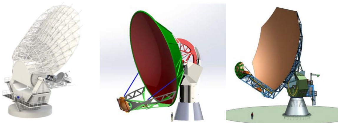
Figure 13 – Additional ngVLA Antenna Concepts. Left: CPI/Vertex Antennentechnik, Center: Calian Technologies/NRCC, Right: OHB/MT Mechatronics.
