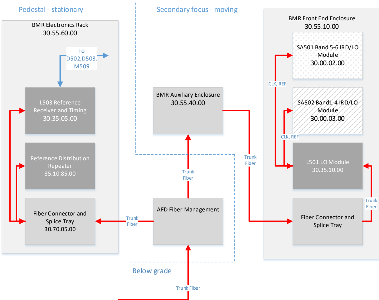
Figure 34 - LRT subsystem components at the Antenna Station. Dark shaded blocks are ATF or RTD line replaceable units, hatched blocks are Antenna Electronics modules with ATF subsystem shop replaceable units (LO modules) within. Light gray shaded blocks are Antenna Electronics elements with fiber optic pass-through. (Red=fiber optic connection)
