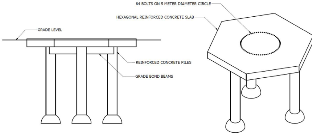
Figure 40 - Antenna foundation supports. Note that site grade is approximately level with the pad, and the piles extend below grade. The 64 1.75" diameter bolts on a 16.896' [5150mm] circle form the primary interface to the antenna pedestal.
