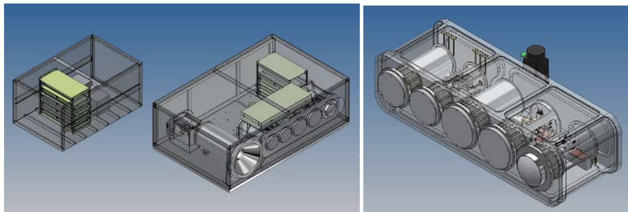
Figure 19 - Left: Front End component packaging at the antenna secondary focus. Band selection and focus are achieved with a dual-axis translation stage. Integrated receiver packages are located in close proximity to cryostats, minimizing the analog signal path length (Section 7.4.3). Right: Bands 2-6 are housed within a single cryostat.
