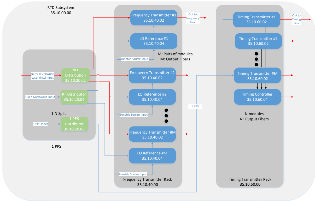
Figure 31 - LO Reference and Timing: Central Distribution (RTD) Transmitters only.
