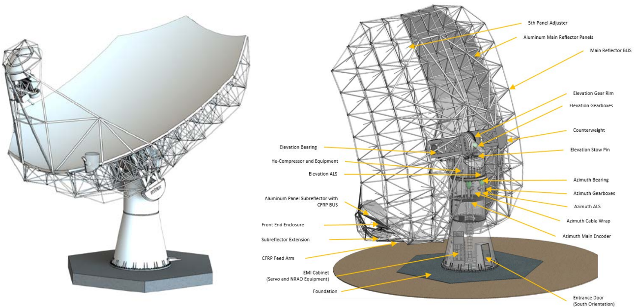
Figure 14 – Selected conceptual design of the 18m antenna, courtesy of mtex antenna technology gmbh.
