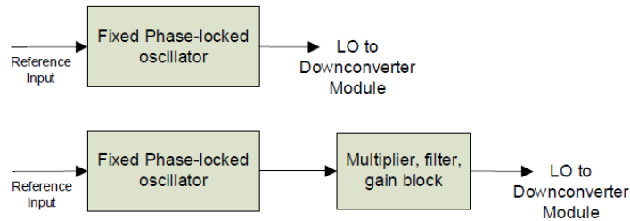
Figure 33 - Antenna LO architecture of independent frequency oscillators for each IRD downconverter module. A total of 19 LO modules are included in the design.
