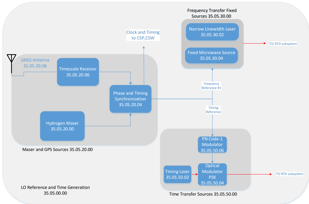
Figure 30 - LO Reference & Timing Generation (RTG) subsystem block diagram. Note that the Frequency Transfer Offset Sources are a placeholder for possible centrally generated antenna offsets.
