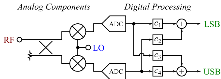
Figure 21 – A sideband-separating mixer with a numerically implemented IF quadrature hybrid using calibrated complex-gain coefficients. Details are conceptual only. The hybrid will be replaced by a 90-degree phase shift on the quadrature LO in the ngVLA implementation, and the complex gain coefficients for sideband separation are implemented in the DBE.
