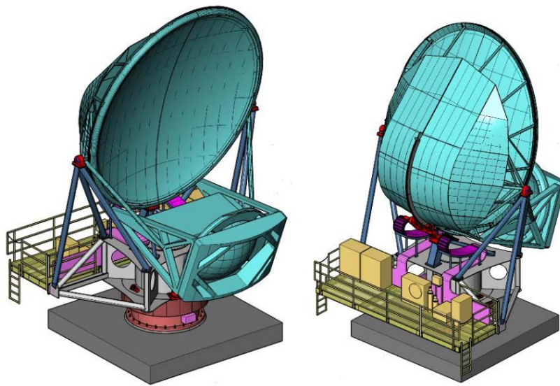
Figure 16 - NRCC conceptual design of the 6m short baseline array antenna.
