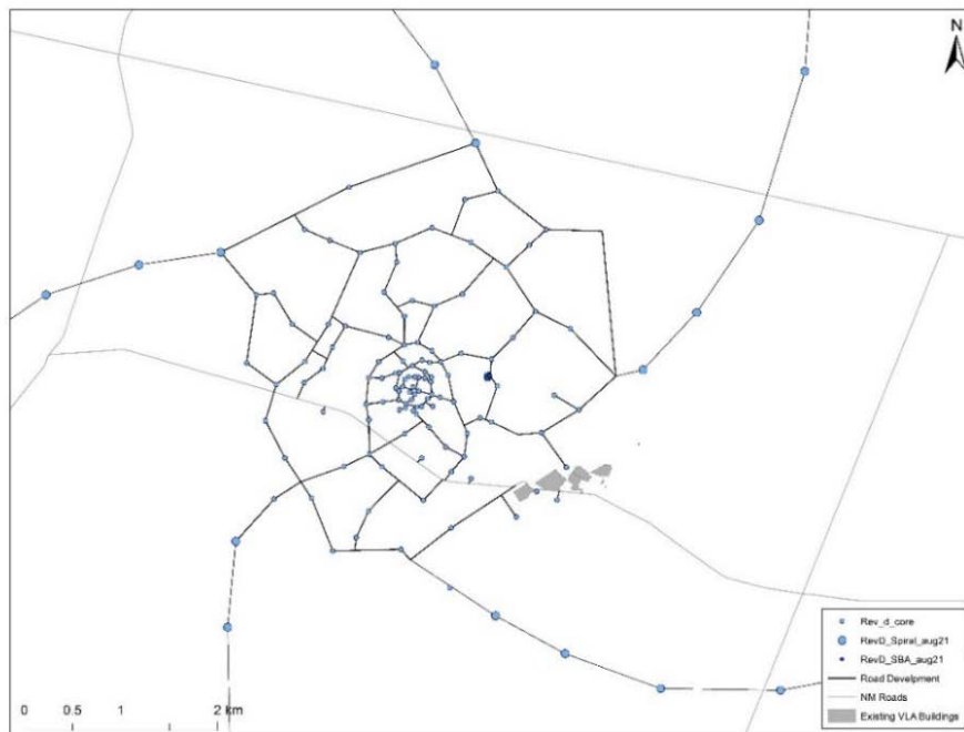
Figure 41 - Road and trench configuration for the ngVLA central core and spiral arm antennas.
