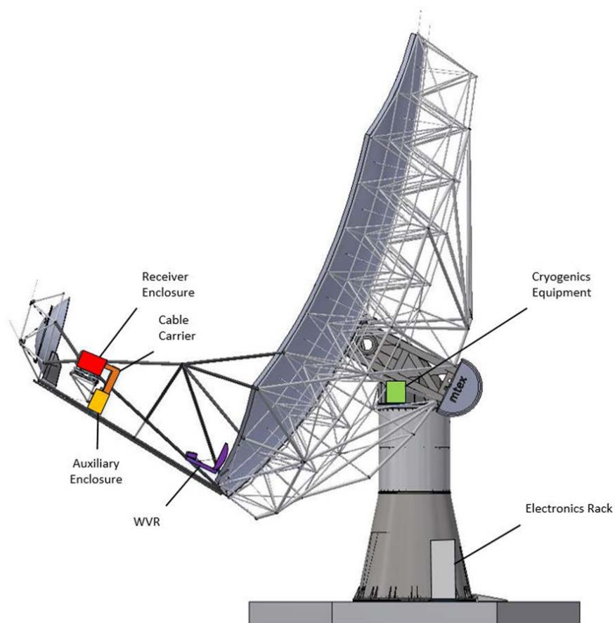
Figure 26 - Antenna electronics locations for mechanical packaging and environmental control.
