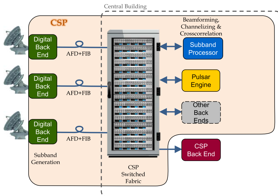
Figure 35 - CSP High-level block diagram.
