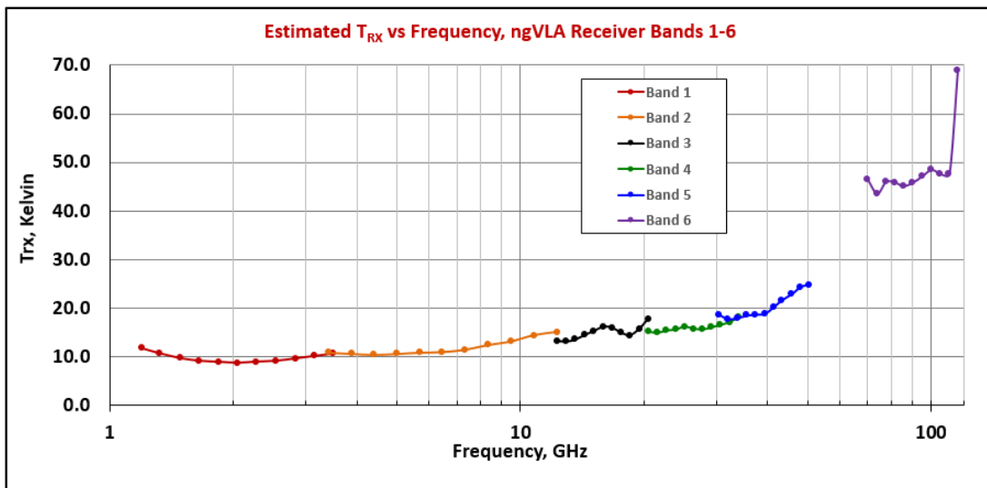
Figure 17 - Receiver Temperature for the ngVLA 6-band receiver concept.
