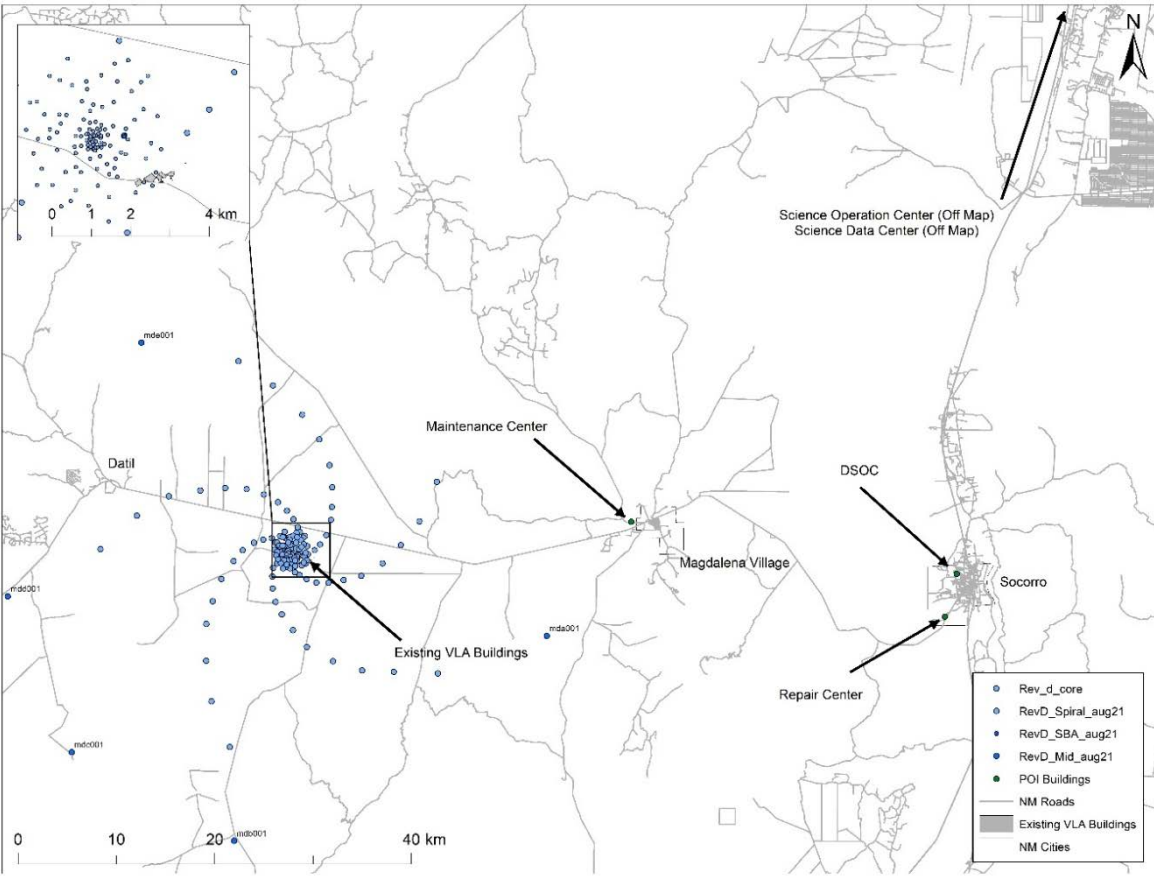
Figure 39 - A site context diagram for infrastructure and buildings. The array infrastructure sub-system must connect all antenna sites to necessary services (power, fiber, roads). The sites of various buildings are also shown for context. The Maintenance Center, Repair Center and Array Operations Center (existing DSOC) are elements of the Operations Buildings package. The Science Operations Center and Science Data Center are off map.
