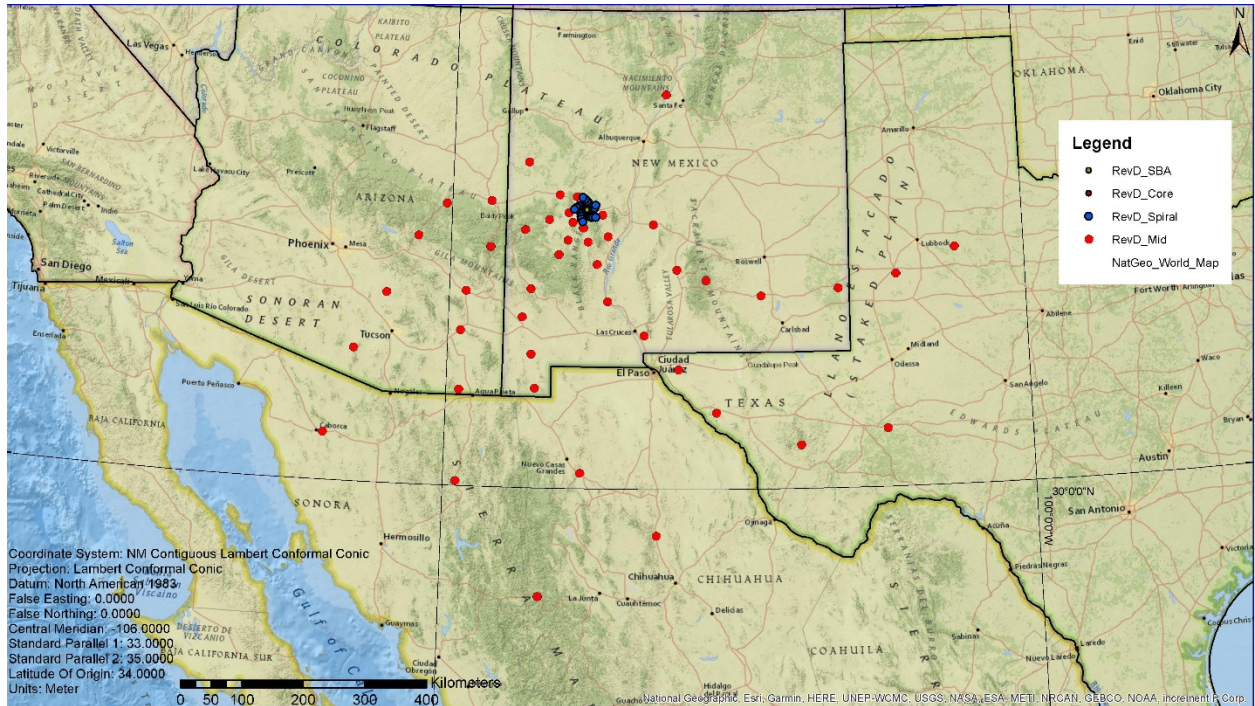
Figure 11 - ngVLA Main Array Configuration Rev D mid-baseline antenna sites in the southwestern US and northern Mexico. These antenna positions are still notional, but are representative for performance quantification and cost estimation.
