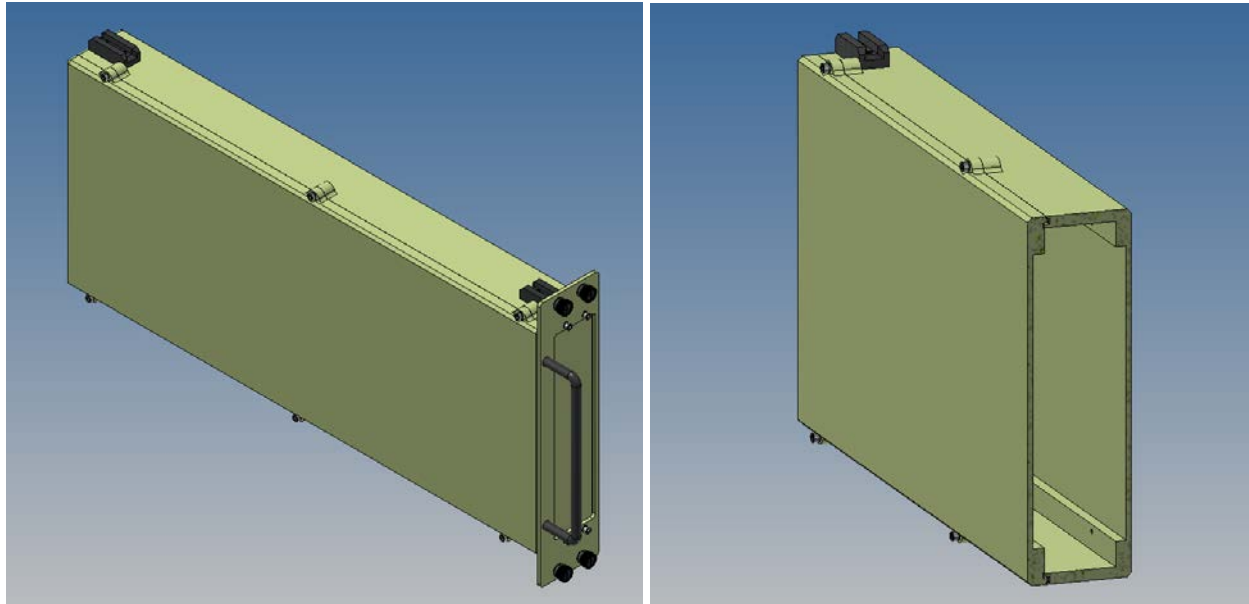
Figure 27 - 500 Series ARCS Module, closed and cross section views
