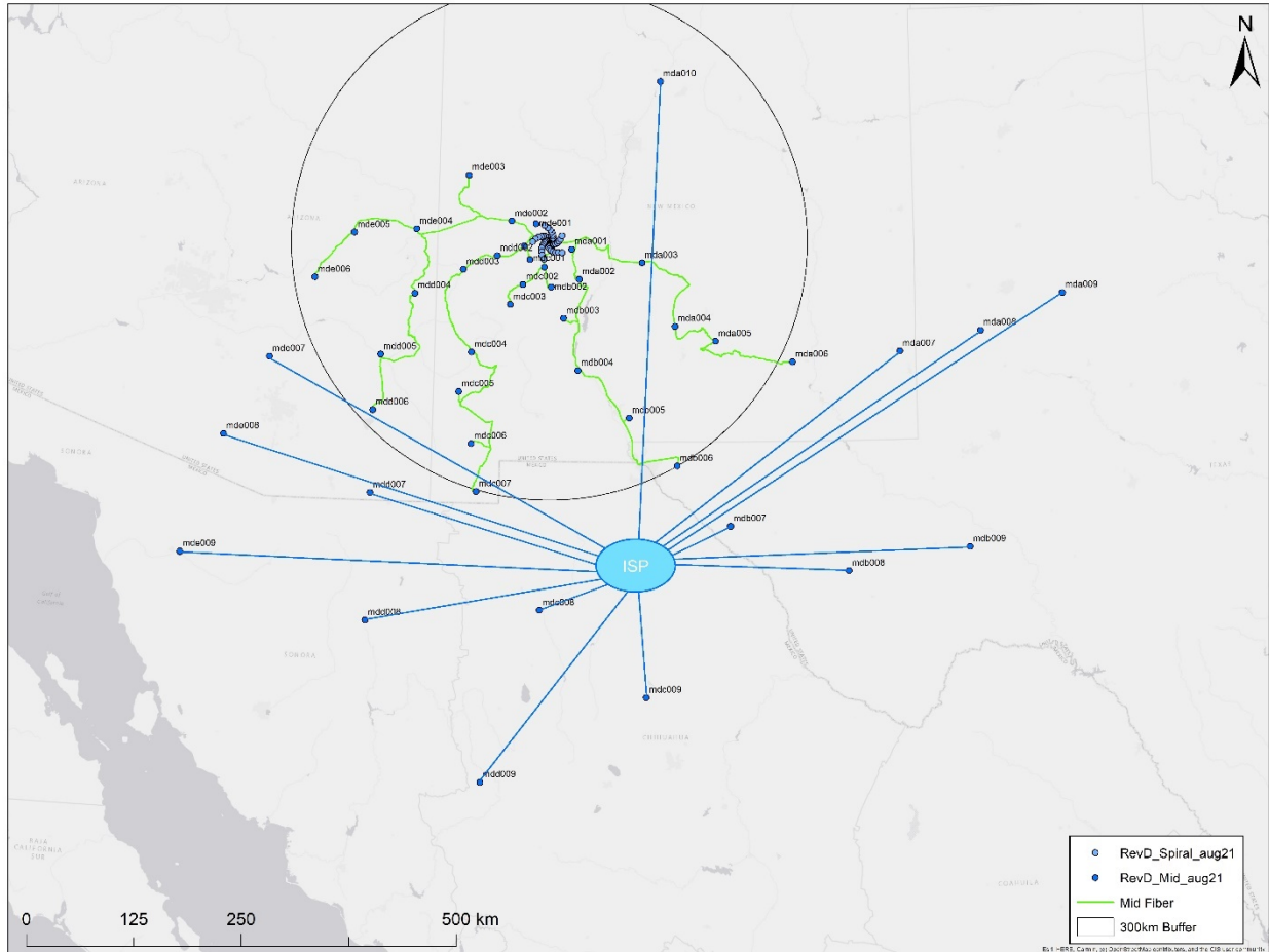
Figure 36 - Preliminary fiberoptic system layout for mid-baseline stations of the Main Array. Antennas within the core and spiral arms are direct point-to-point connections over ngVLA operated fiber. Mid-baseline stations within ~300km are connected over dedicated fiber links with repeater infrastructure housed at each antenna station. Mid-baseline stations outside the ~300 km radius, and all long-baseline stations, rely on leased bandwidth provided by network operators.
