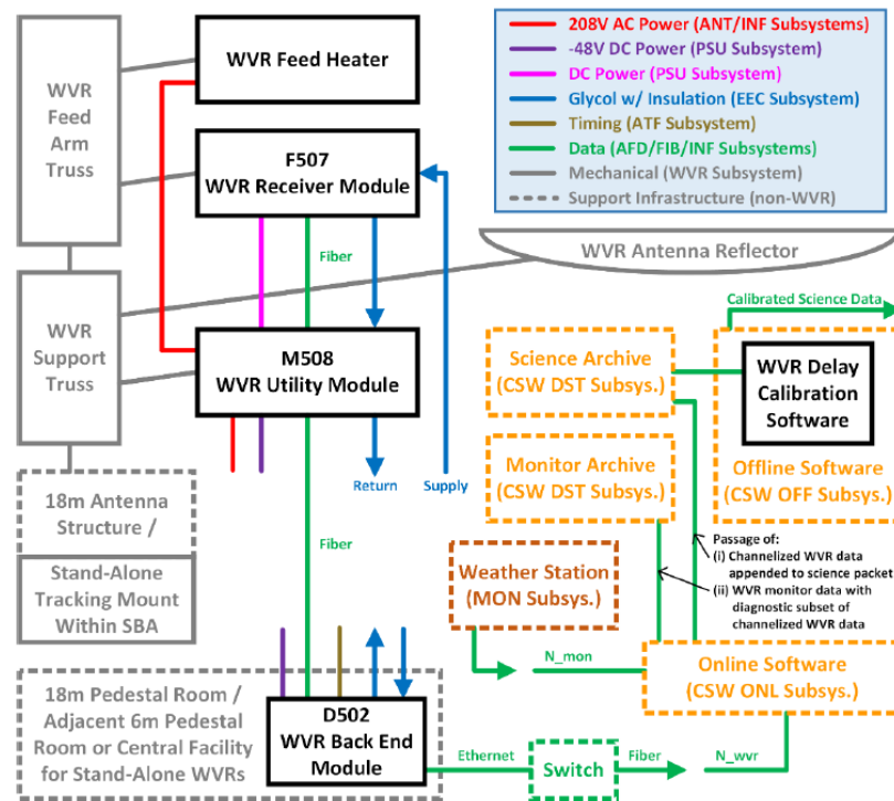
Figure 24 - WVR system block diagram and interfaces.
