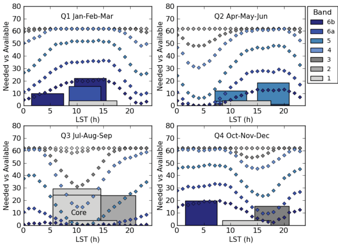
Figure 2 – Comparing the times needed (histograms) to the times available (lines) in Year 1 of the Reference Observing Program. The colors encode the bands and apply to both histograms and lines. The abscissa is the Local Sidereal Time for the Core subarray. The ordinate is the number of LST passes needed vs available. Three months offer no more than 6000 \text{ h} / (4 \times 24 \text{ h}) passes, thus \sim 62 passes.
