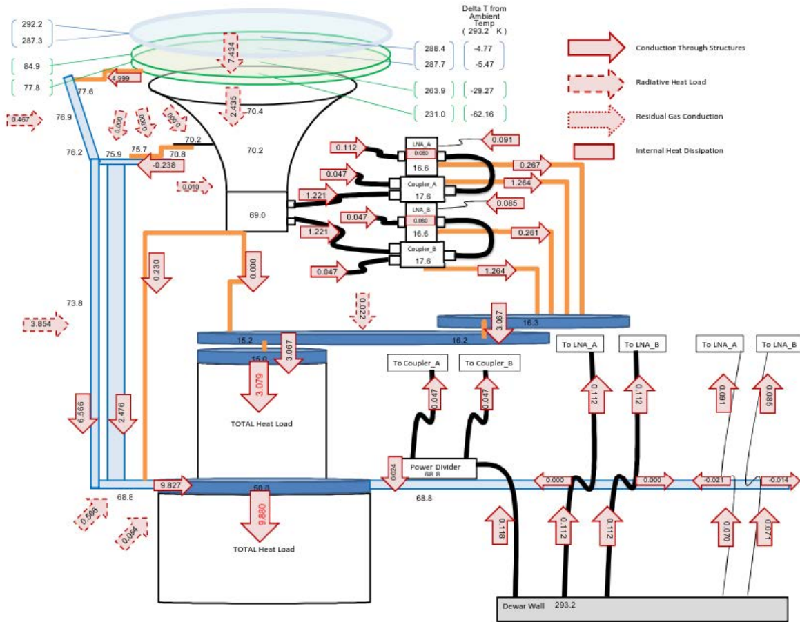
Figure 25: Graphical representation of heat flow results from modeling of the Band I receiver in Cryostat A, using the ThermXL® analysis tool. In this particular case, an ambient of 20°C and a cryostat pressure of 10 -6 mbar was assumed, and 1 st and 2 nd stage temperatures of 50 K and 15 K, respectively.
