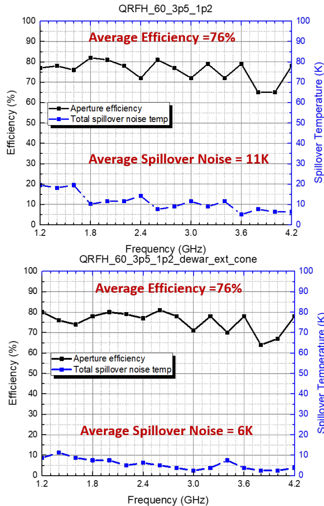
Figure 4: Simulated aperture efficiency of the Caltech feed horn with a dual-offset Gregorian shaped antenna. The external shield serves to redirect the backlobe away from the ground and toward cold sky, reducing spillover noise. Antenna elevation in these cases is 90 degrees (zenith).
