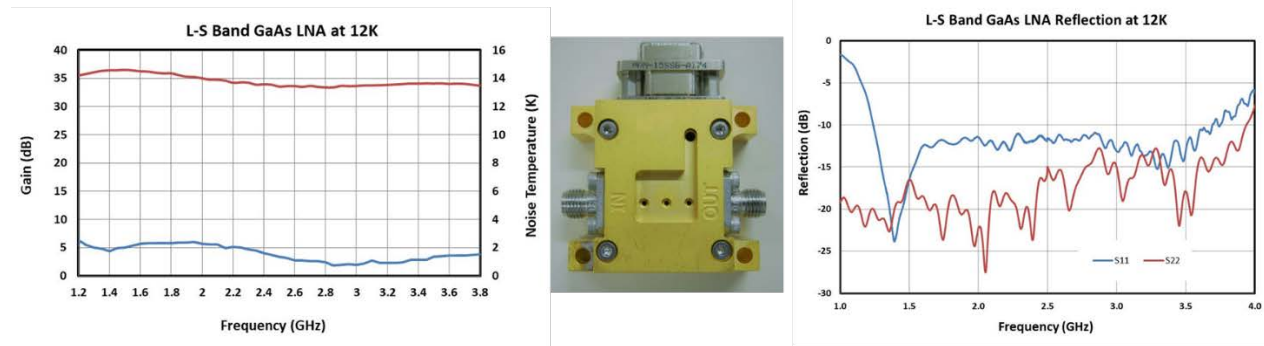
Figure 36 – NRC HAA prototype GaAs HEMT LNA for ngVLA Band 1 (center photo), flanked by plots of gain and noise performance (L) and input/output port return loss ®. Gain is on the red trace, noise temperature on the blue trace.
