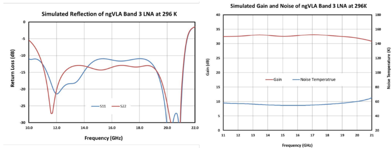
Figure 37 – Simulated ambient temperature gain and noise performance ® and input/output port return loss (L), NRC HAA InP HEMT LNA design for ngVLA Band 3. Input return loss is > 11 dB over the full band.
