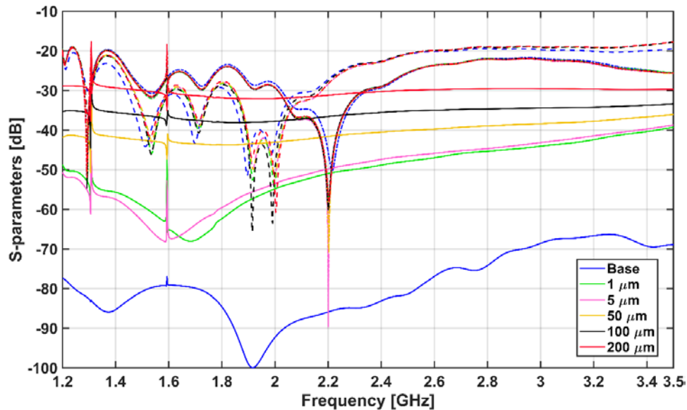
Figure 8: S_{11} (dash), S_{22} (dash-dot), and S_{21} (solid) for the EMSS QRFH with a 2-port balun. One ridge is offset by the distance given in the legend, degrading port isolation and enhancing the trapped-mode resonances.
