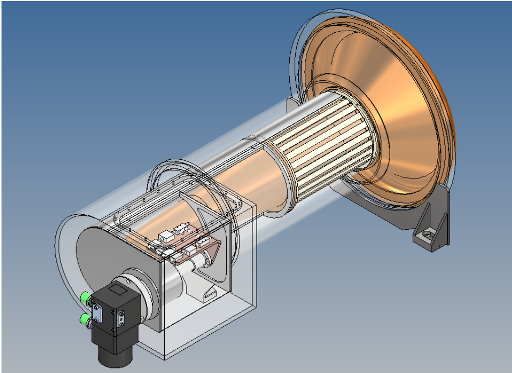
Figure 19: Cryostat 'A' (Band 1). The flared horn section of the QRFH is outside the vacuum space at ambient temperature. This reduces the cryostat mass, while adding a very small amount of additional noise.
