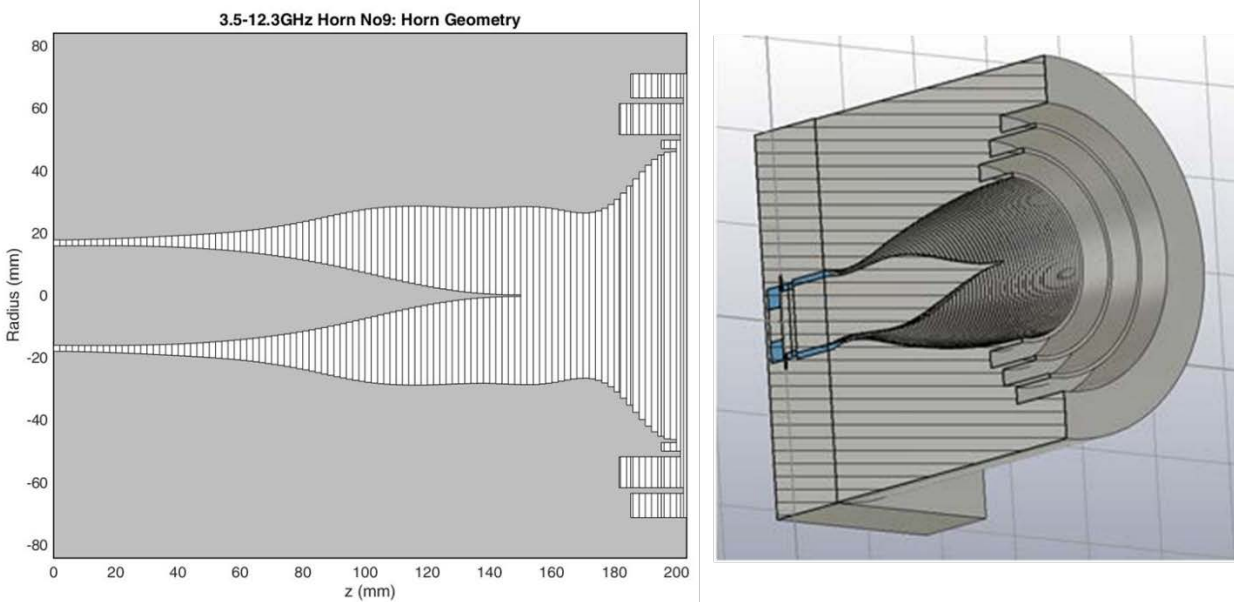
Figure 12: LAR Band 2 ‘bullet’ feed horn concept. The OMT needed for driving the coaxial waveguide input on the left side is not shown here; a preliminary 4-port balanced design from LAR was \sim 200 mm long.
