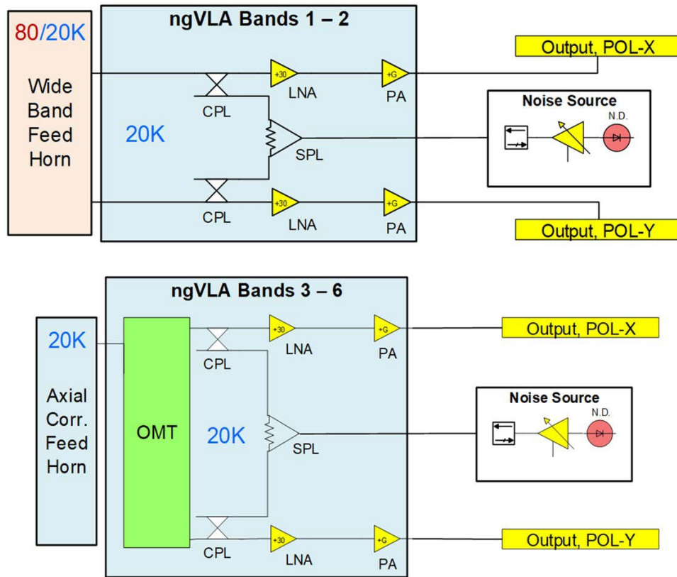
Figure 18: ngVLA Front End receiver block diagrams, Bands 1 & 2 (top) and Bands 3–6 (bottom). Note that the OMT is integral with the feed horn on Bands 1–2, but is a separate waveguide component on Bands 3–6.
