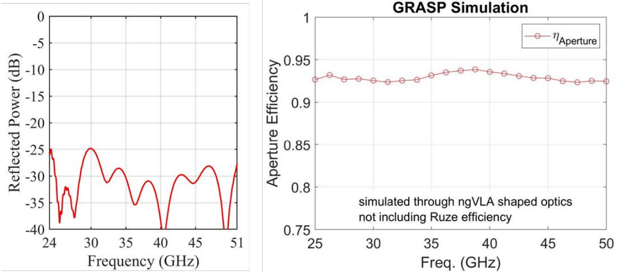
Figure 40 – (Top) NRC HAA octave-bandwidth corrugated feed horn, with a quad-ridged circular waveguide output to match the OMT. (Bottom) Simulations of input match (L) and aperture efficiency \eta_{\text{Aperture}} , using the ngVLA antenna optics.
