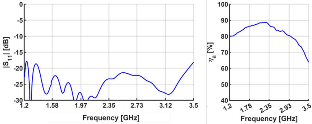
Figure 6: Simulated output return loss and aperture efficiency of the EMSS Band I feed horn concept. The ngVLA conceptual antenna optics were assumed for the calculation.
