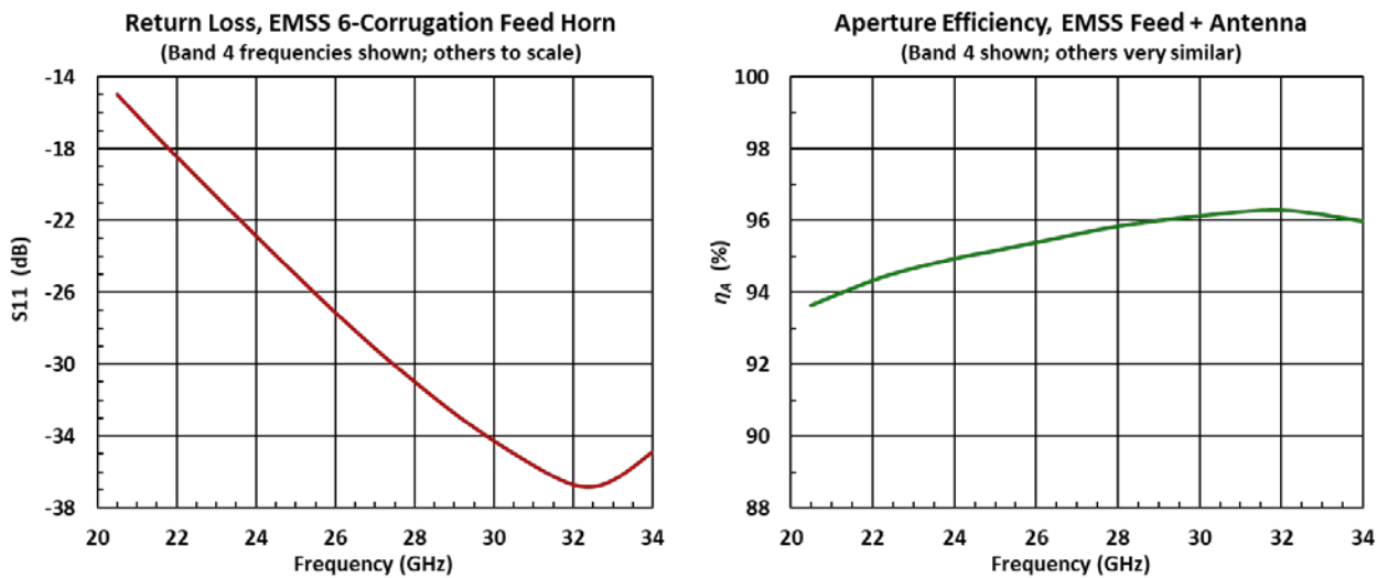
Figure 15: Simulated return loss and aperture efficiency versus frequency of the EMSS corrugated feed horn, using the ngVLA conceptual antenna optics. Performance at Bands 3, 5, and 6 is nearly the same, other than the frequency scale. Aperture efficiency shown does not include ohmic loss or roughness effects from the reflectors.
