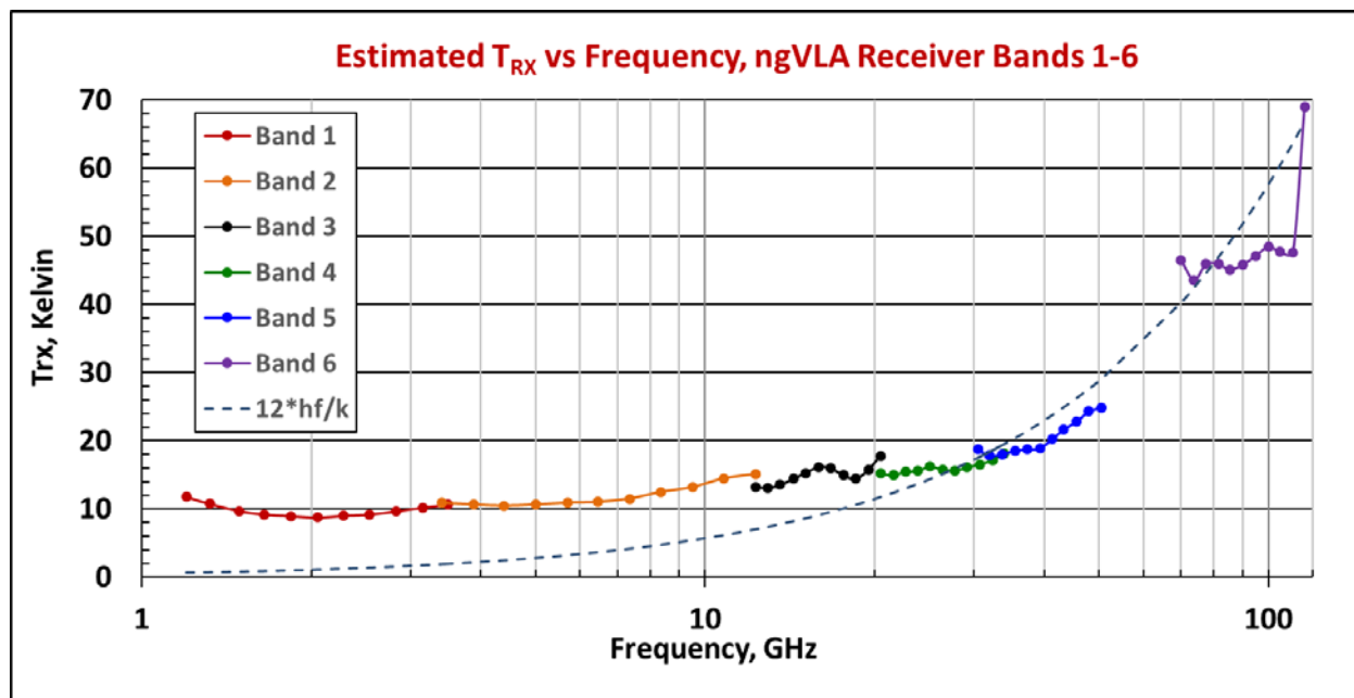
Figure 28: Receiver noise temperatures, ngVLA Bands 1–6.
